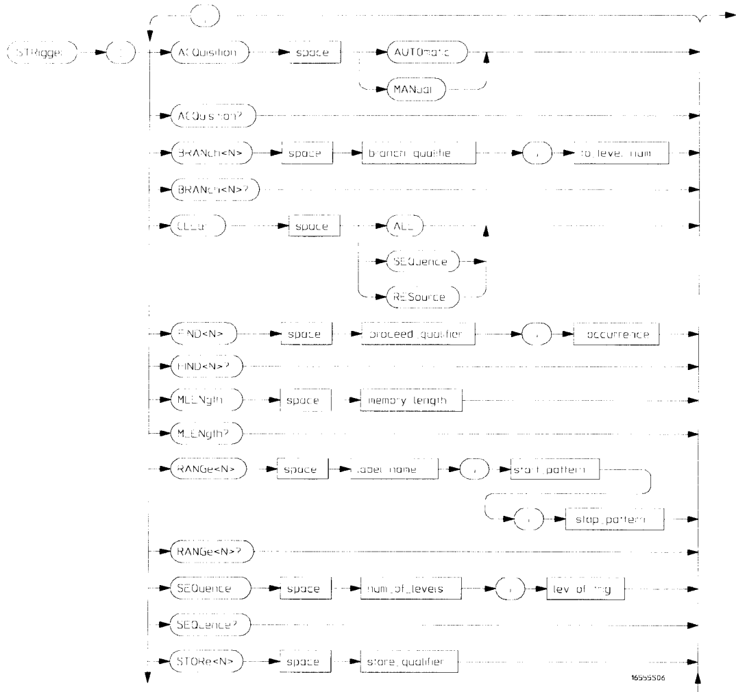
STRigger Subsystem Syntax Diagram
