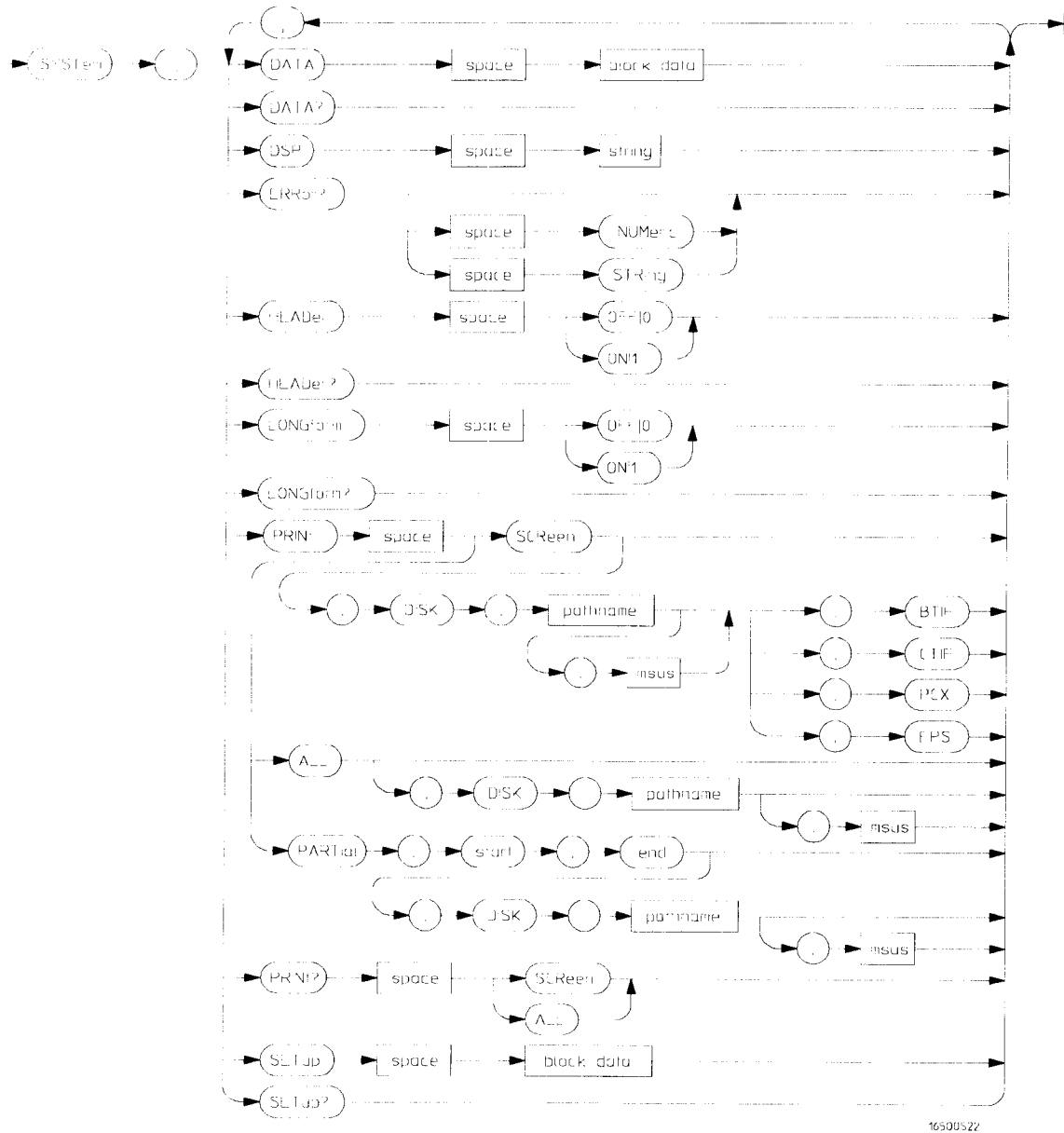
System Subsystem Commands Syntax Diagram
