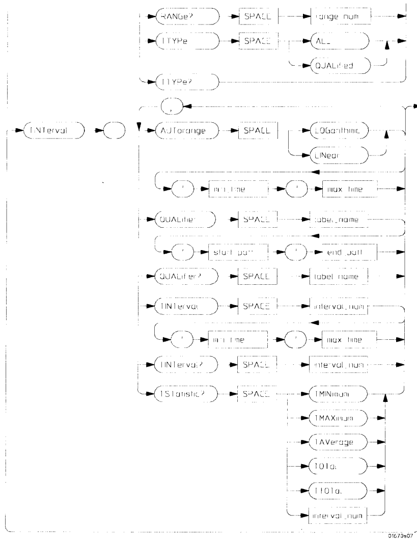
SPA Subsystem Syntax Diagram (continued)
