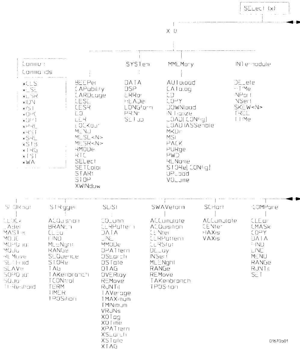
HP 1670A-Series Command Tree
