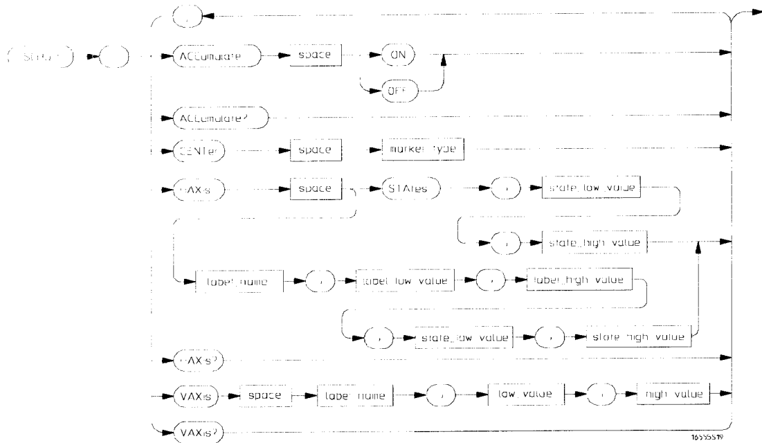
SCHart Subsystem Syntax Diagram
