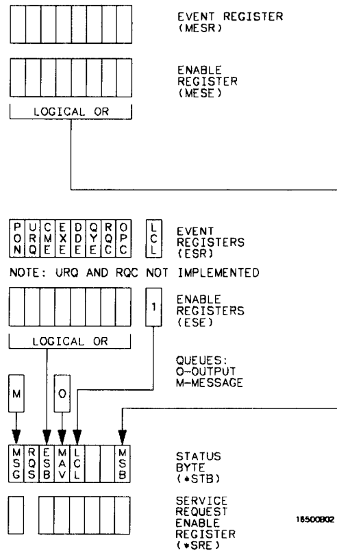
Status Byte Structures and Concepts
