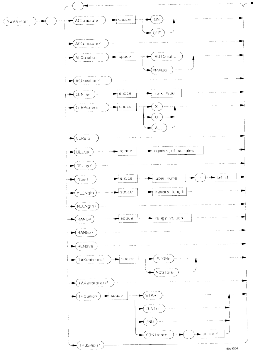
SWAVeform Subsystem Syntax Diagram
