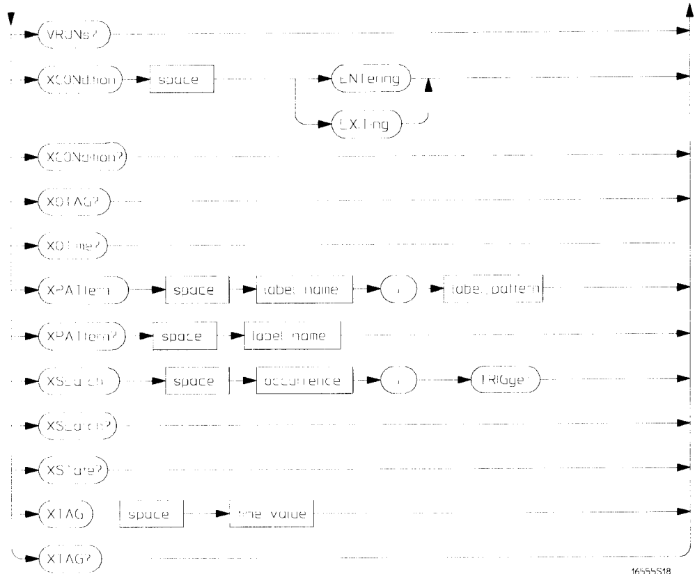
TLISr Subsystem Syntax Diagram (continued)
