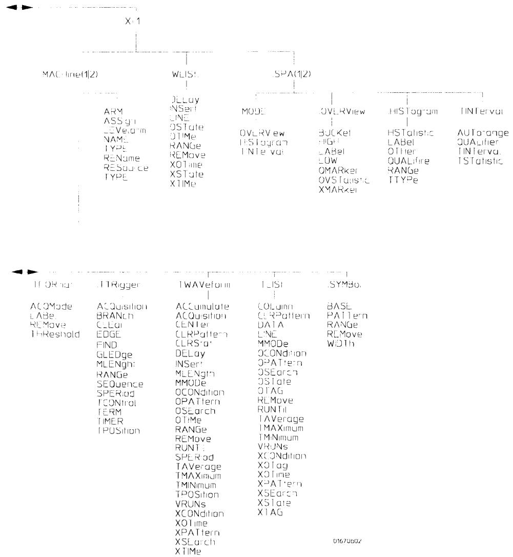
HP 1670A-Series Command Tree (continued)
