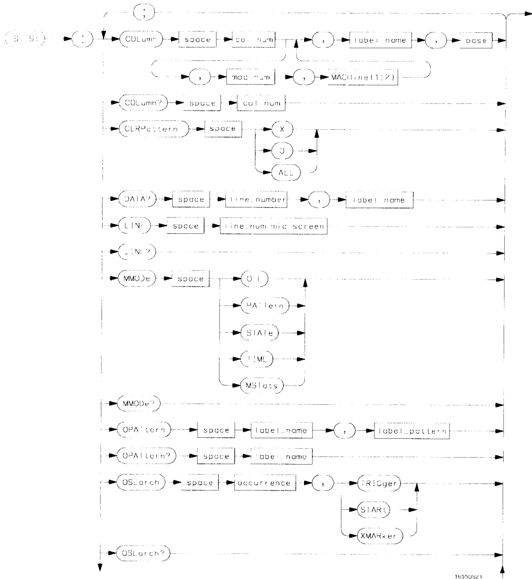
SLISL Subsystem Syntax Diagram
